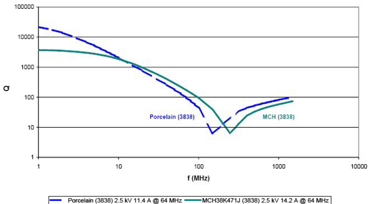
Q vs. Frequency 470 pF @ 25 °C
