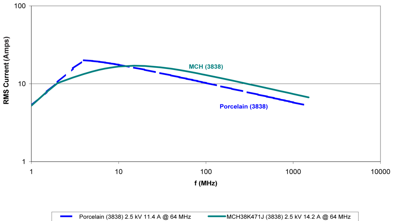
Current Rating (IRMS) for 470 pF at 60 °C Rise
